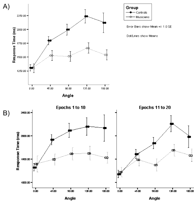
Figure 3. A , Mean RTs (error bars \pm 1 SE of mean) as a function of angle between the paired forms of 3DMR task. The classical behavioral signature of 3DMR task, in which RT increase linearly as a function of angle between the forms, was evident only in nonmusicians. B , Mean RTs (error bars \pm 1 SE of mean) as a function of angle between the paired forms of 3DMR task during epochs 1–10. C , Mean RTs (error bars \pm 1 SE of mean) as a function of angle between the paired forms of 3DMR task during epochs 11–20.
