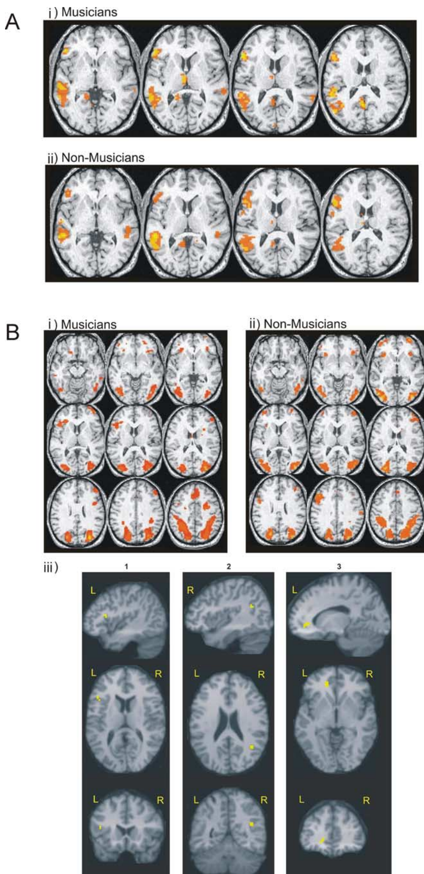
Figure 2. A , Brain activations in musicians and controls during the assessment of verbal intellectual ability. Bi–Bii , Activations resulting from within-group random effects analyses for ( i ) musicians and ( ii ) nonmusicians at z-slice levels used by Sergent et al. (1992) to describe the sight-reading neural network. Top row, Broca's area in left hemisphere activated in Musicians only; middle
